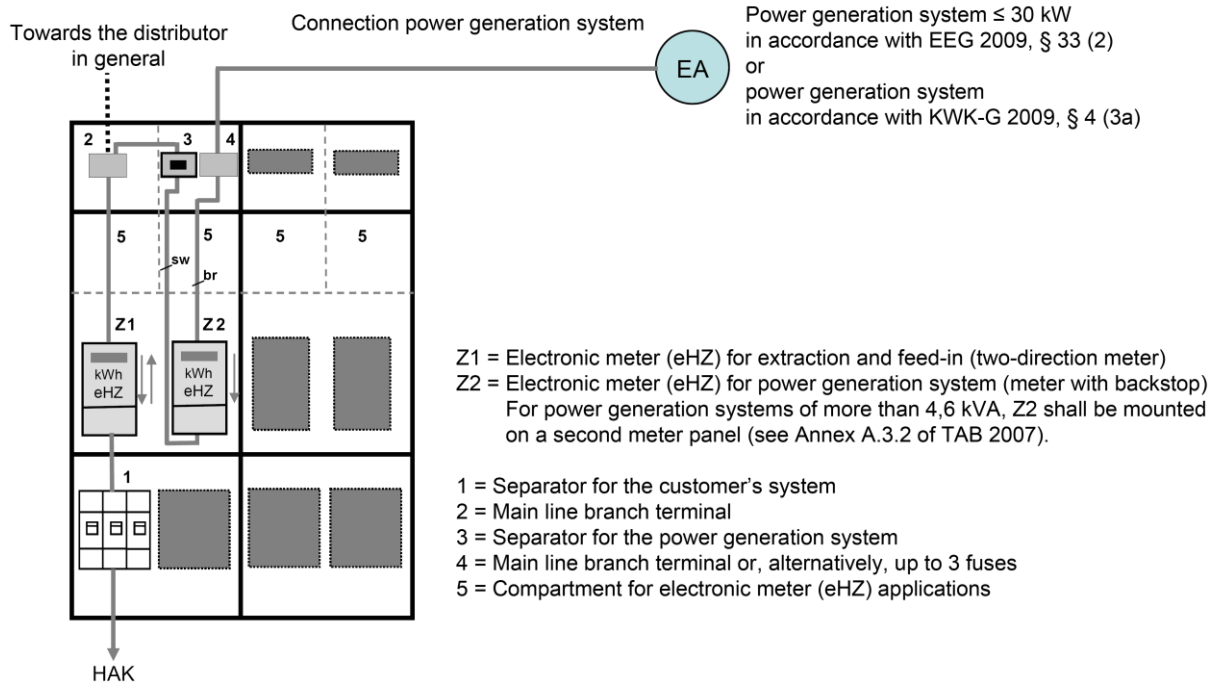
Figure C.7 — Connection variant for a central eHZ meter panel with BKE-I
